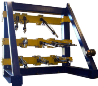
SEAT BELT ANCHORAGE
